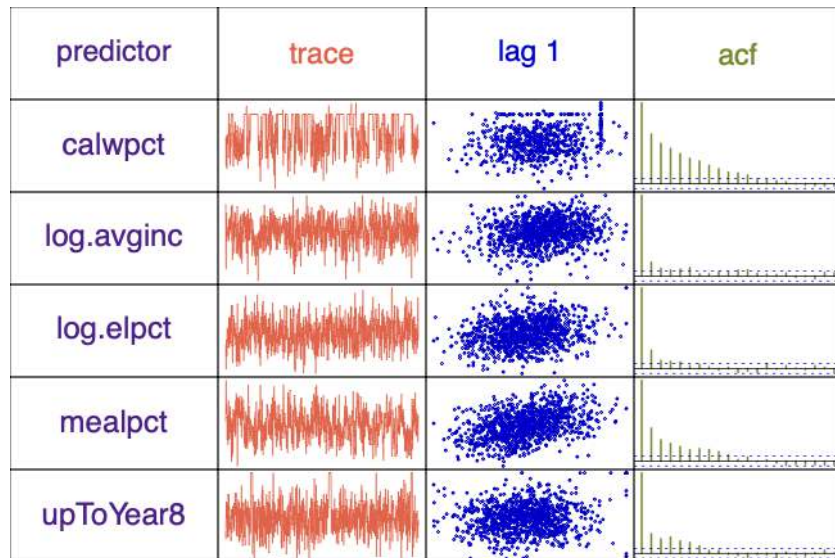
Figure 8: The graphic produced by the command checkChains(fit6) for the ganselBayes() fit object fit6 . The Figure 2 caption provides full details on checkChain() graphics.
