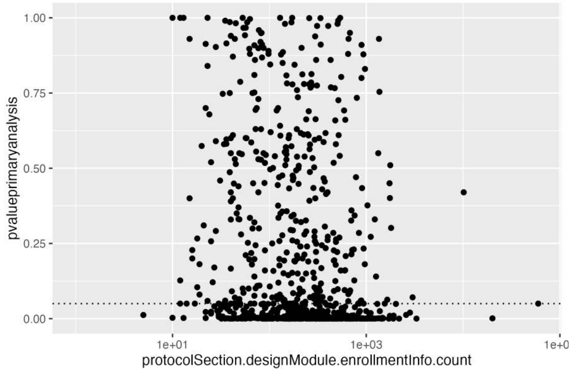
Figure 8: phase23_paed_p_values
