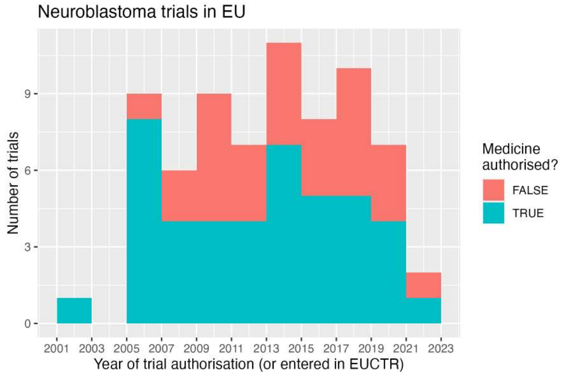
Figure 9: HistogramNBtrials
