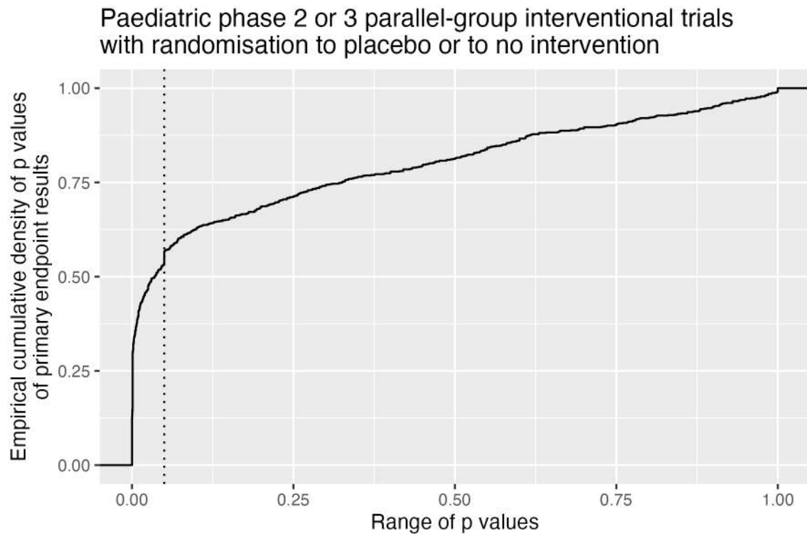
Figure 7: phase23_paed_p_values
