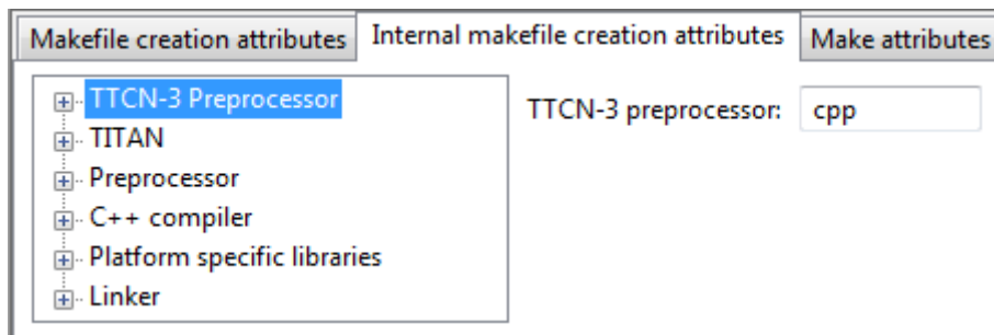
Figure 41. TTCN-3 preprocessor
