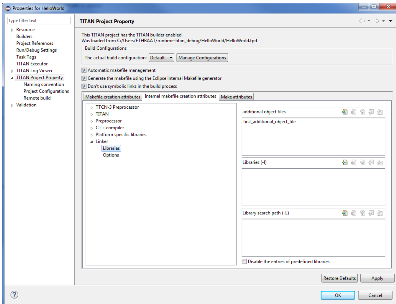
Figure 52. Linker libraries
