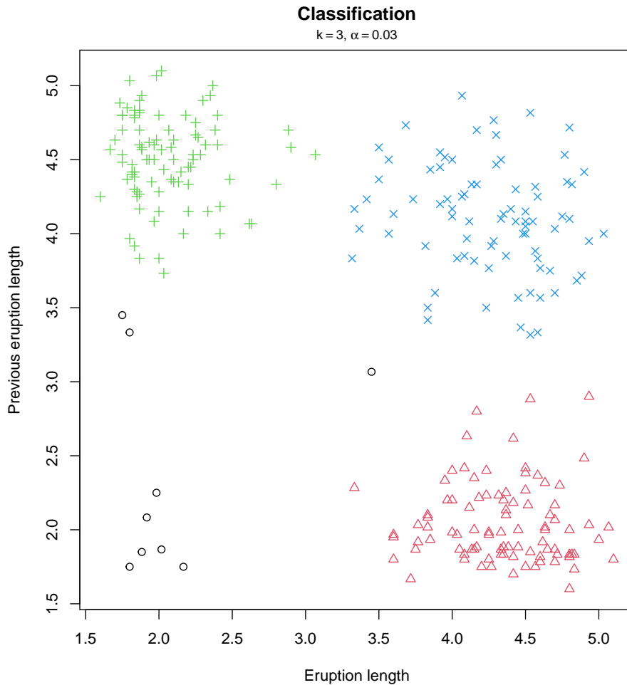
Figure 1: Trimmed k -means results with k = 3 and \alpha = 0.03 for the bivariate Old Faithful Geysers data. Trimmed observations are denoted by the symbol “o” (a convention followed in all the figures in this work).
