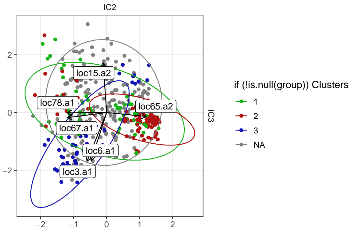
Figure 12: ICA with 2 axes of the Crohn dataset, colored by k-Xi clustering with 95% confidence ellipses.
