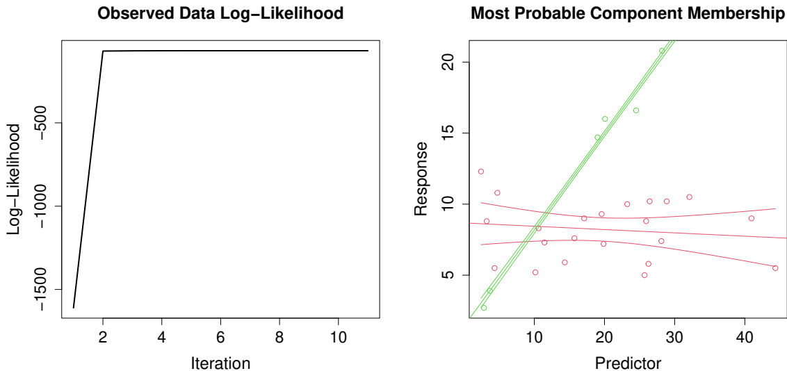
Figure 10: The GNP data fitted with a 2-component parametric EM algorithm in mixtools . Left: the sequence of log-likelihood values, L_{\mathbf{x}}(\boldsymbol{\theta}^{(\ell)}) ; Right: the fitted regression lines with 99% Working-Hotelling Confidence Bands.
