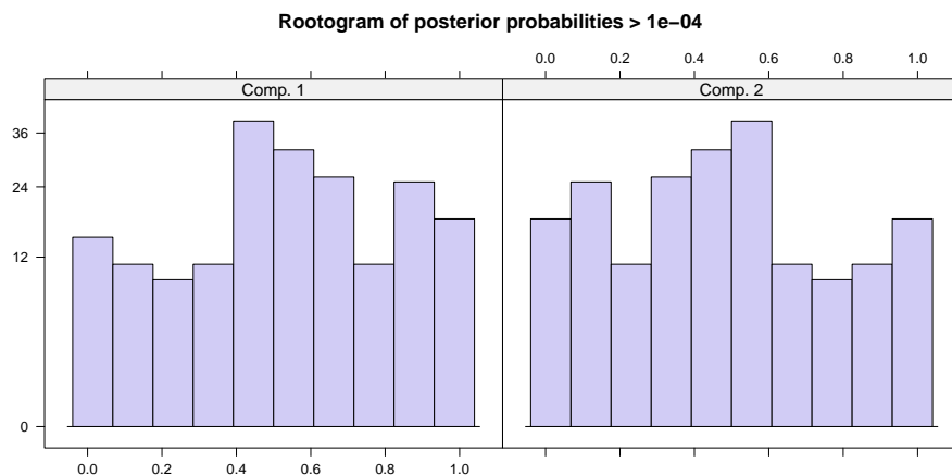
Figure 3: plot(m2)
