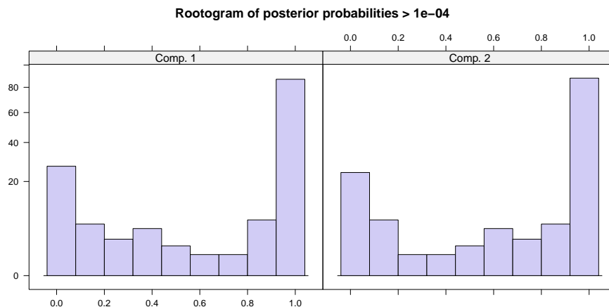
Figure 4: plot(m3)
